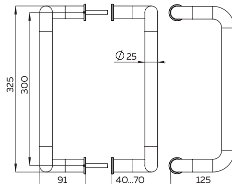
PULL.PH25/300.25 INOX 304
