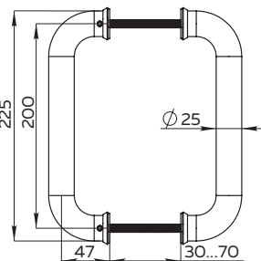
PULL.PH25/300.21 INOX 304
