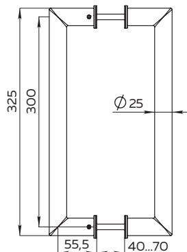
PULL.PH25/300.23 INOX 304
