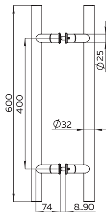
PULL.PH32/600.45 INOX 304
