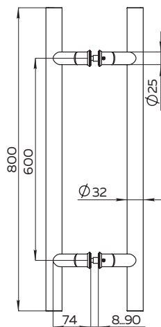
PULL.PH32/800.45 INOX 304
