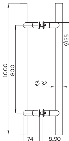
PULL.PH32/1000.45 INOX 304
